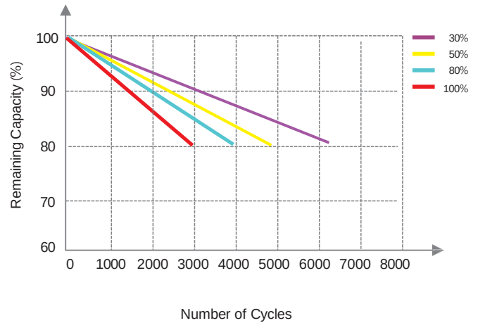
Different DOD Discharge Cycle Life Curve(1C)
